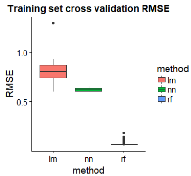
Figure 8. RMSE of each model during cross validation.
