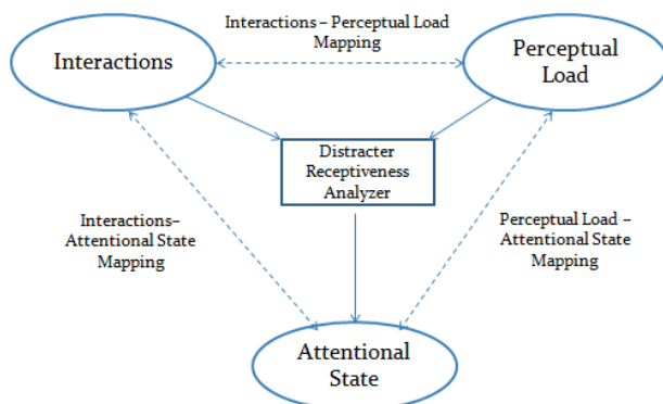
Figure 3: System Architecture
